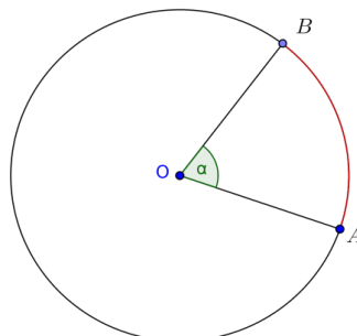
Figura 30 – Arco central
